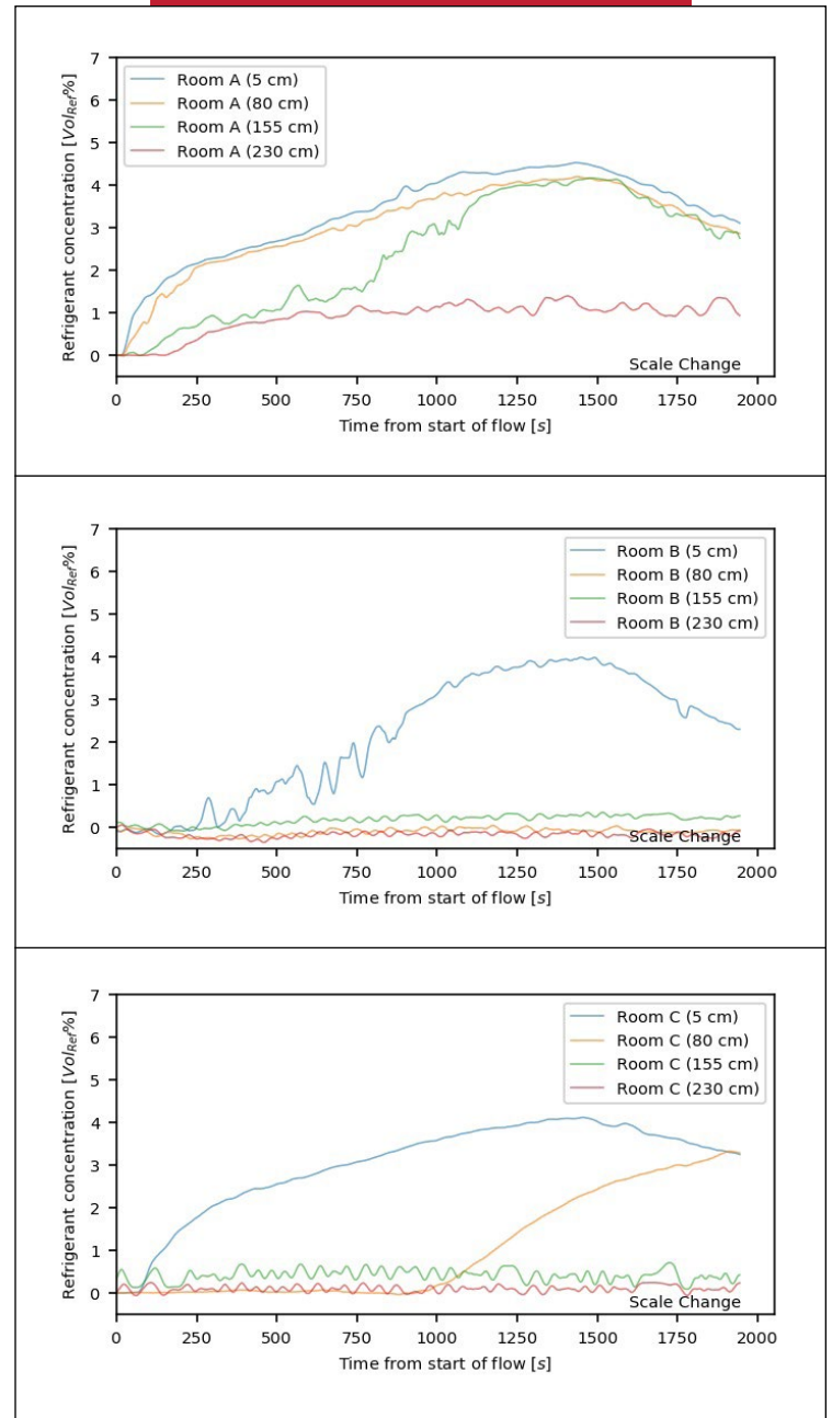
Figure 6 – Larger clearance concentrations
