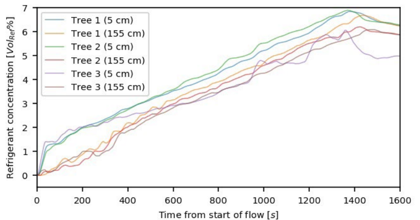
Figure 2 - Refrigerant concentration in Room A
