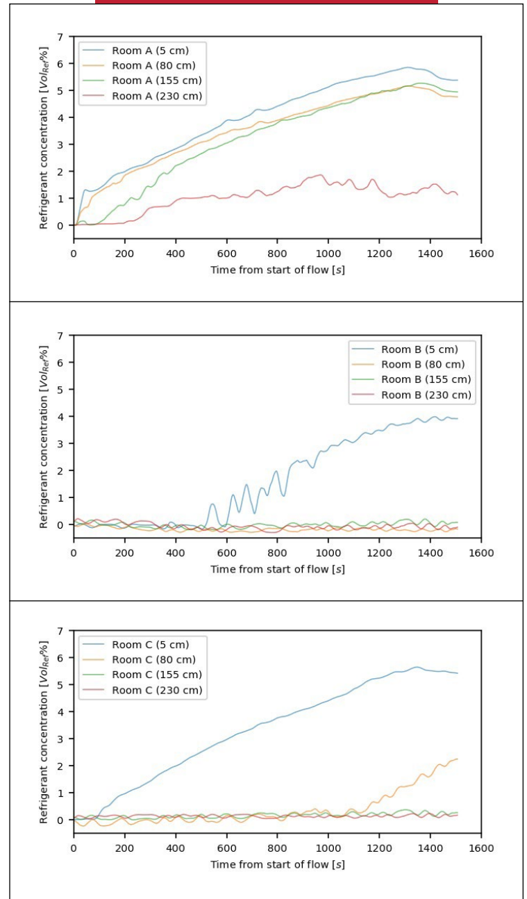
Figure 5 – Small clearance concentrations
