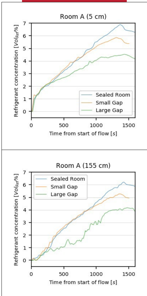
Figure 7 - Door gap summary
