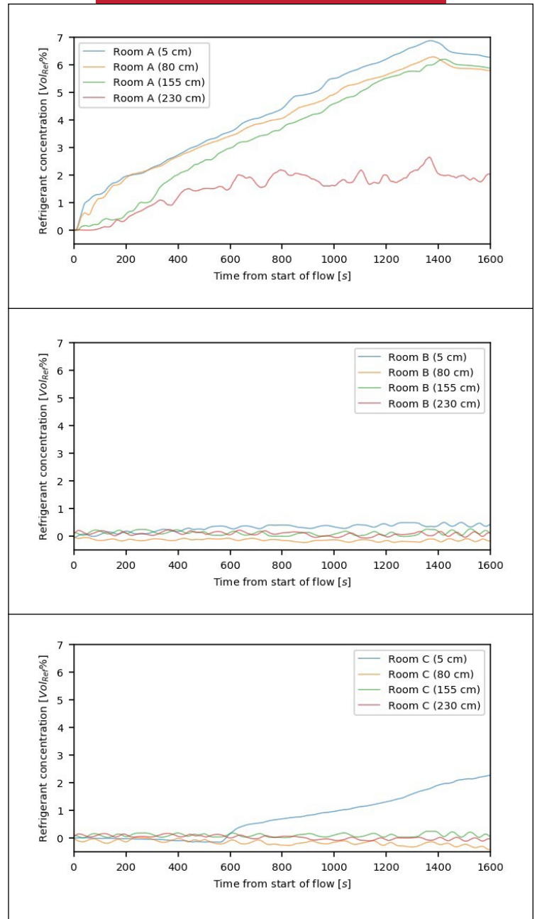
Figure 4 - Room tightness concentrations
